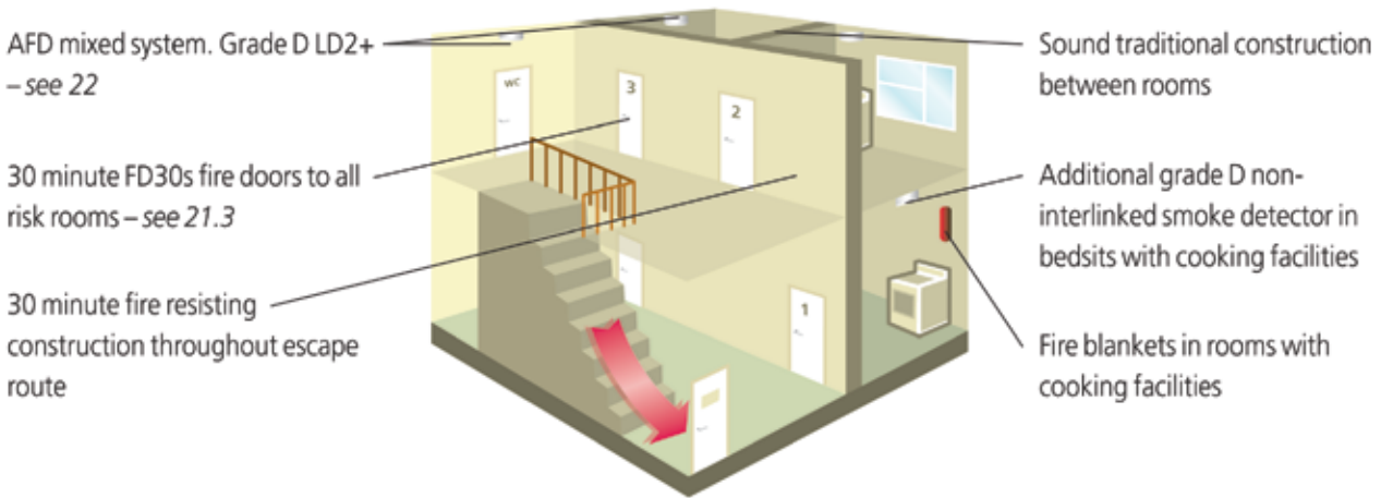
figure D7: bedsit-type HMO, two storeys
