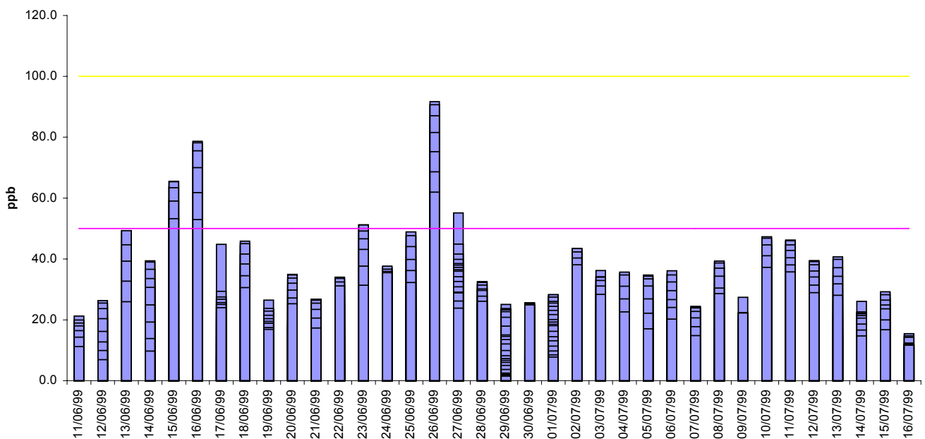
Ozone (O 3 ) Running 8 Hour Mean Low up to 50ppb Moderate up to 100ppb
