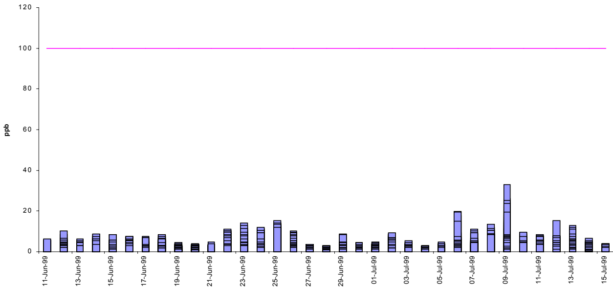
Sulphur Dioxide (SO 2 ), 15 minute mean Low up to 100ppb
