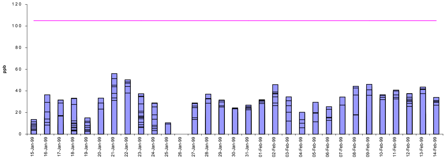
Nitrogen Dioxide (NO 2 ) Hourly Mean NO 2 Limit=105ppb
